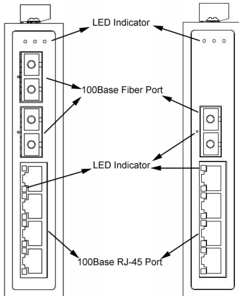
Front Panel of the 4-port 10/100TX + 1 or 2-port 100FX Industrial Switch
