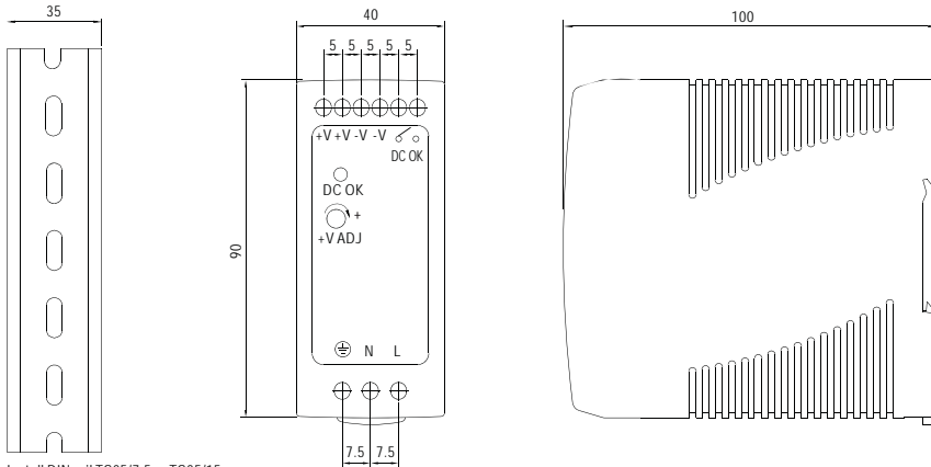
Install DIN rail TS35/7.5 or TS35/15
